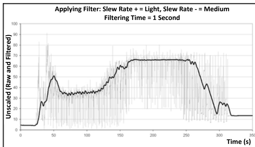
Figure 8: Filtering the RAW Unscaled Signal (1)
