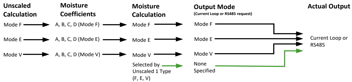
Figure 12: None specified Output Selection
