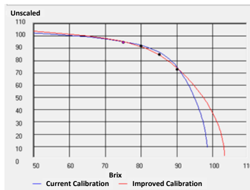
Figure 22: Example of a Good Brix Calibration
