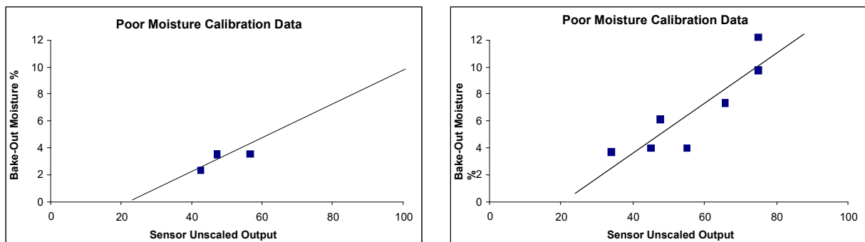
Figure 19: Examples of Poor Material Calibration Points
