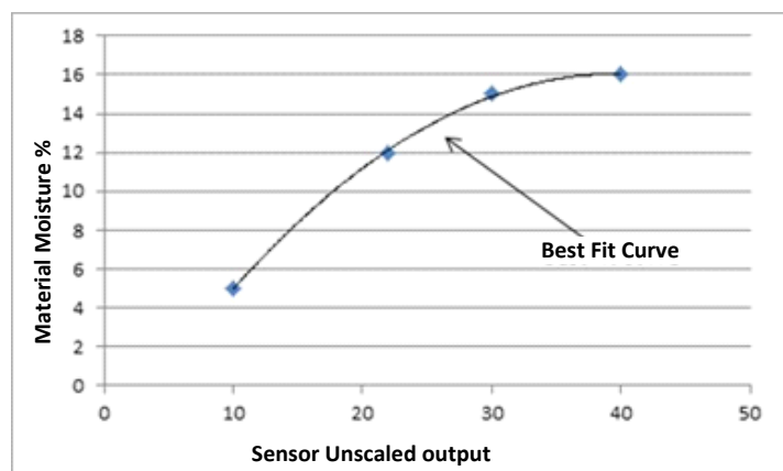
Figure 20: Example of a Good Quadratic Calibration
