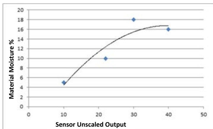
Figure 21: Example of a Bad Quadratic Calibration
