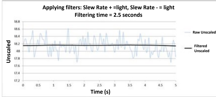
Figure 5: Graph showing the Filtered Signal
