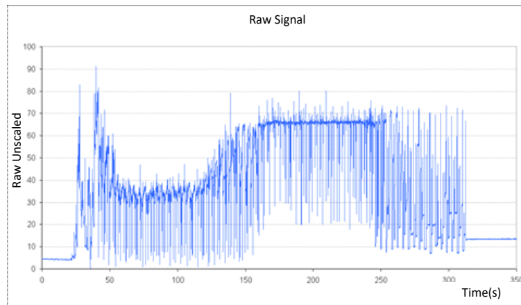
Figure 7: Graph showing Raw Signal during Mix Cycle
