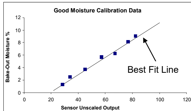
Figure 18: Example of Good Material Calibration
