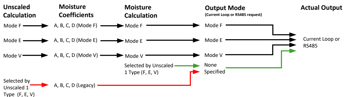
Figure 13: Legacy Output Selection
