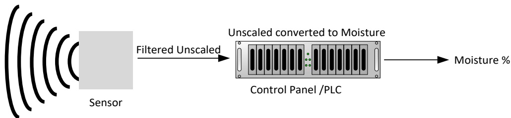
Figure 17: Calibration inside the Control System
