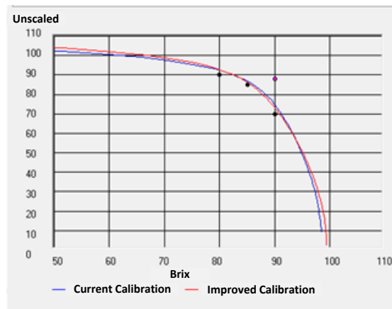
Figure 23: Example of a Bad Brix Calibration
