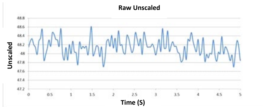
Figure 4: Raw Unscaled Moisture Trace in Flowing Material
