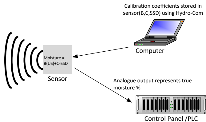
Figure 16: Calibration inside the Sensor
