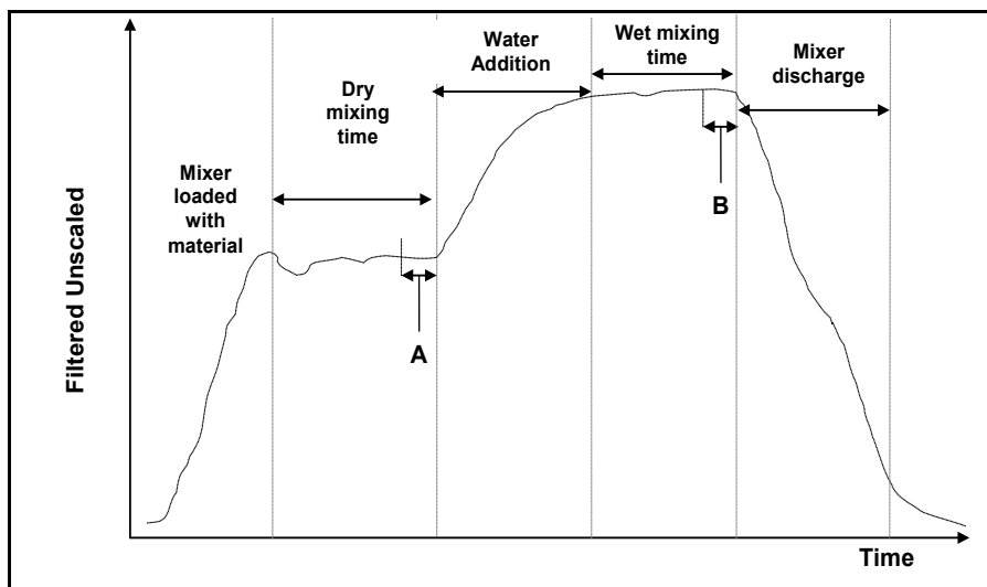
Figure 6: Typical Moisture Curve
