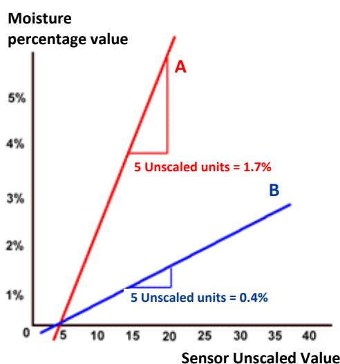
Figure 10: Relationship of Unscaled Values to Moisture
