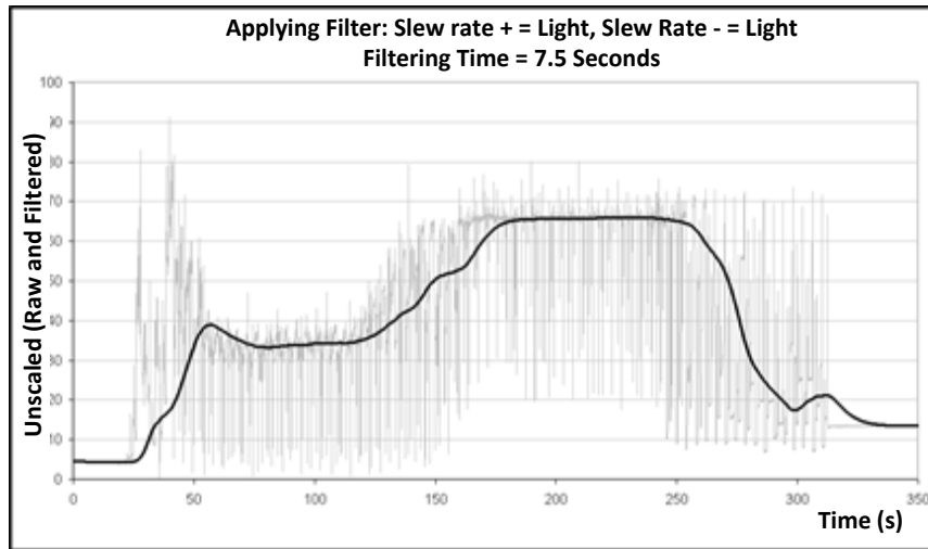
Figure 9: Filtering the RAW Signal (2)
