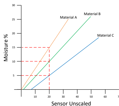
Figure 14: Calibrations for 3 Different Materials
